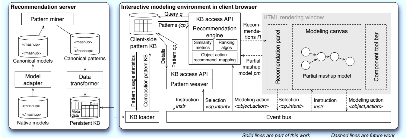
Figure 2: Functional architecture of the composition knowledge discovery and recommendation approach
