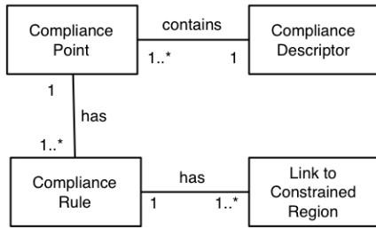
Fig. 5 UML meta model of a compliance descriptor
