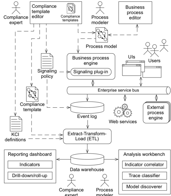
Fig. 2 Event-based compliance management architecture
