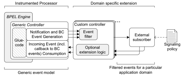
Fig. 8 Architectural overview of the core components of the signaling extension of Apache ODE [15]
